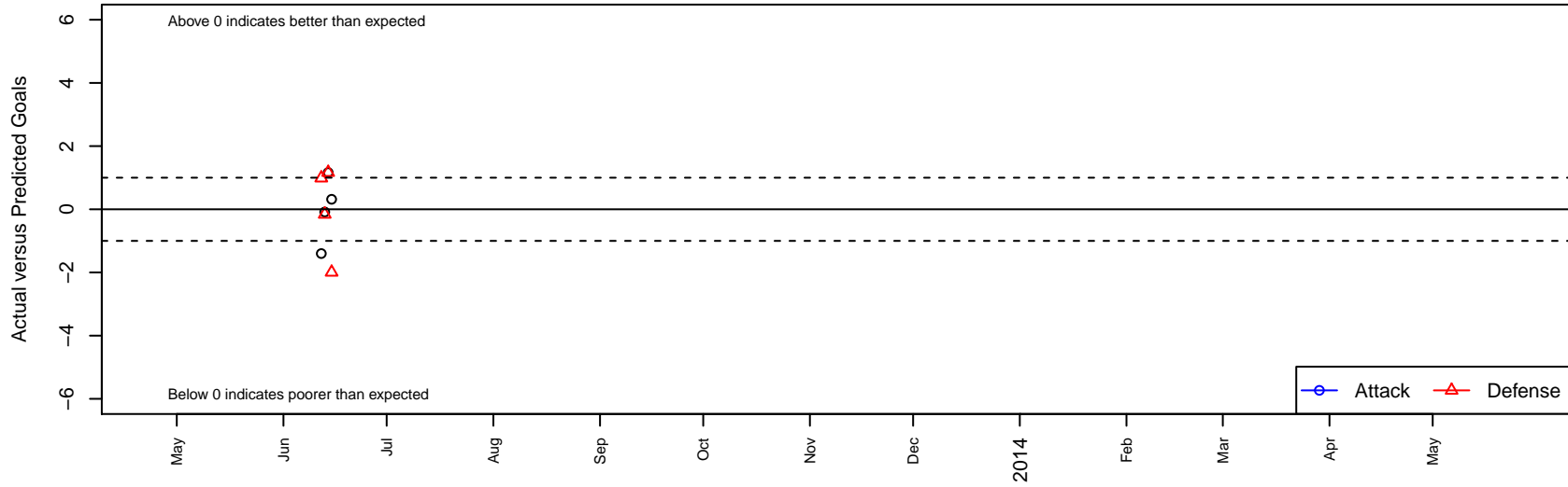
Southbank Excel 00 G99 Dots are actual minus expected GF (blue circles) and GA (red triangles). Blue line is smoothed change in attack strength. Red is smoothed change in defense strength.
